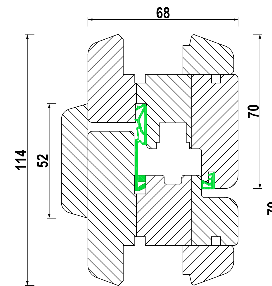
STULP 114mm
